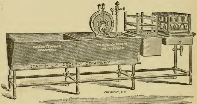
Star Bottle Washing Outfit.
